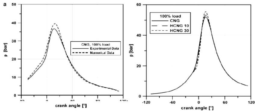
Fig.2 Cylinder pressure as function of the crank angle for CNG at 3000 rpm numerical and experimental results and HCNG 10 ( 10%) and 30 using MBT spark advance for load 100%. [20]
