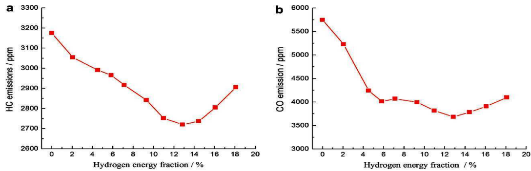
Fig 1 (a) Effect of hydrogen addition on HC emissions at idle and stoichiometric conditions. (b) Effect of hydrogen addition on CO emission at idle and stoichiometric conditions [18]
